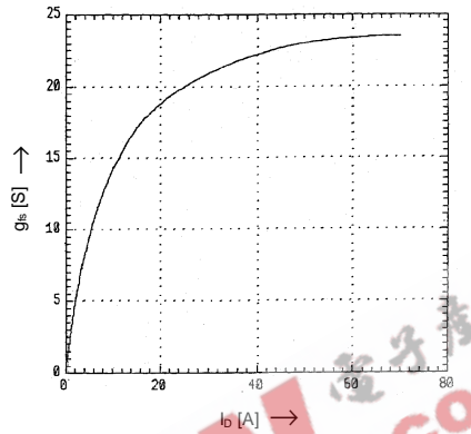
Typical Forward Transconductance vs. I_D
