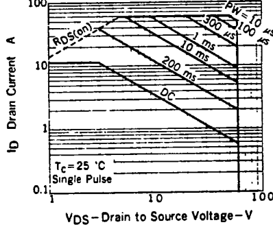
FORWARD BIAS SAFE OPERATING AREA
