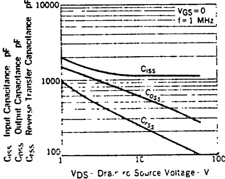
CAPACITANCE vs. DRAIN TO SOURCE VOLTAGE
