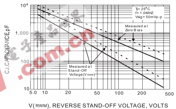
Fig.4 TYPICAL CAPACITANCE
