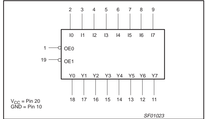
LOGIC SYMBOL – 74F541
