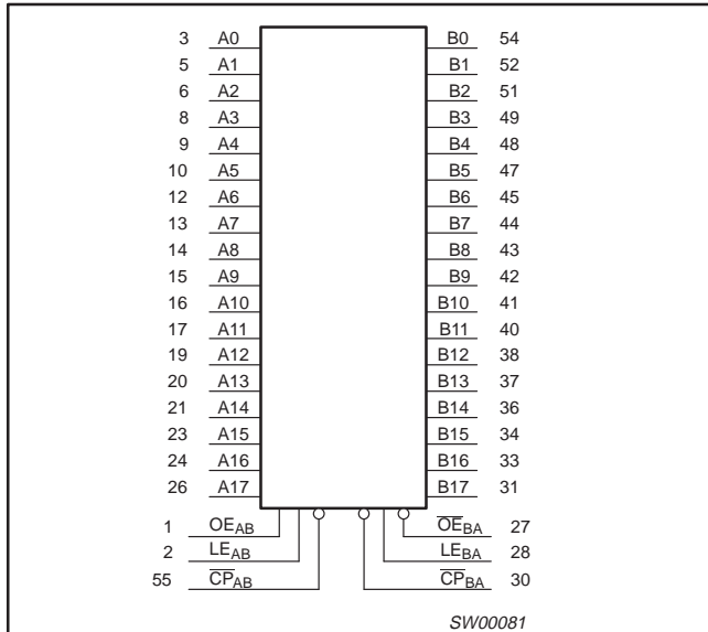
LOGIC SYMBOL
