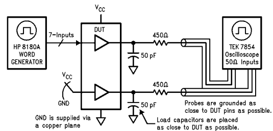
FIGURE 6. Simultaneous Switching Test Circuit
