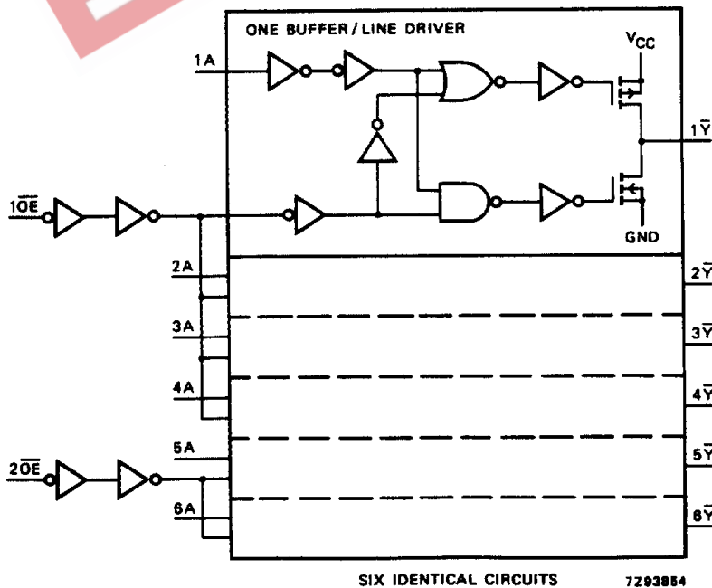
Fig.5 Logic diagram.
