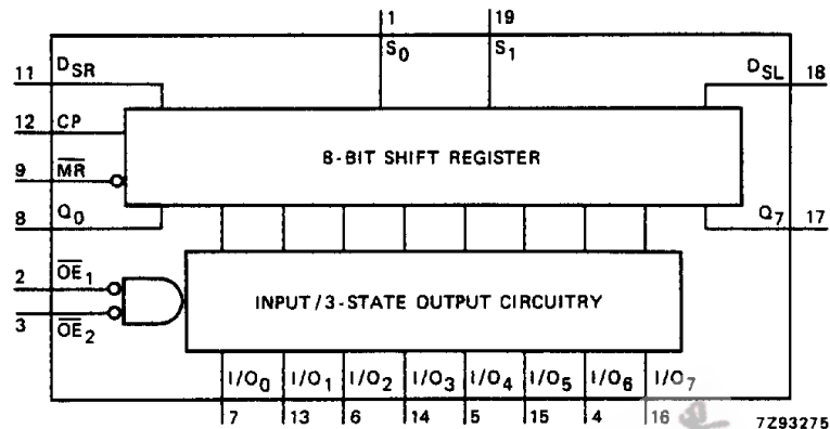
Fig.4 Functional diagram.
