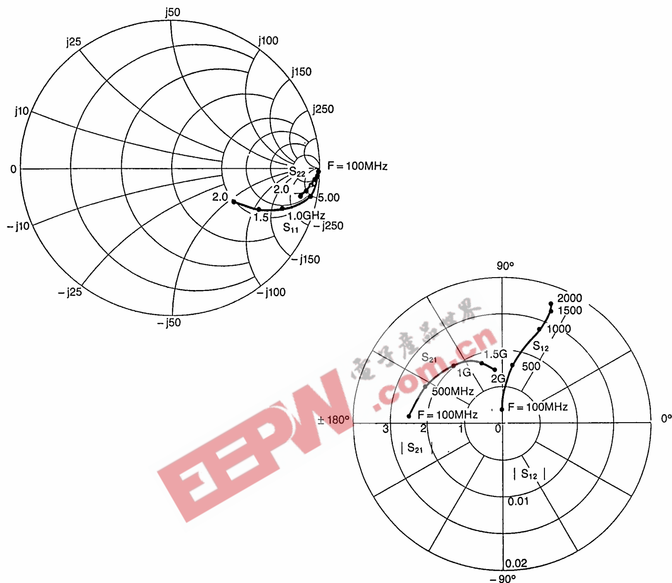
S-Parameter Data of FET 3SK147 (50.0 Ohm reference)
