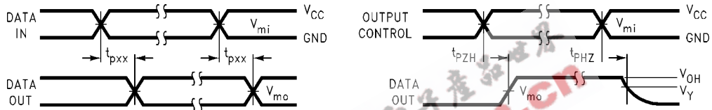
FIGURE 2. Waveform for Inverting and Non-Inverting Functions
