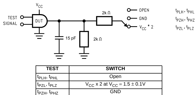
FIGURE 7. AC Test Circuit
