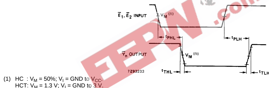
Fig.7 Waveforms showing the enable input ( \bar{E}_n ) to output ( \bar{Y}_n ) propagation delays and the output transition times.
