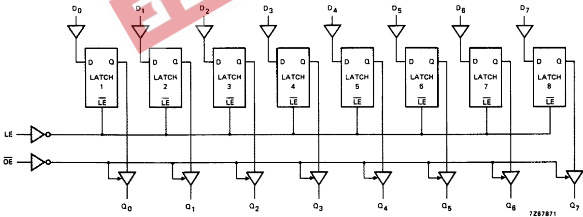
Fig.5 Logic diagram.
