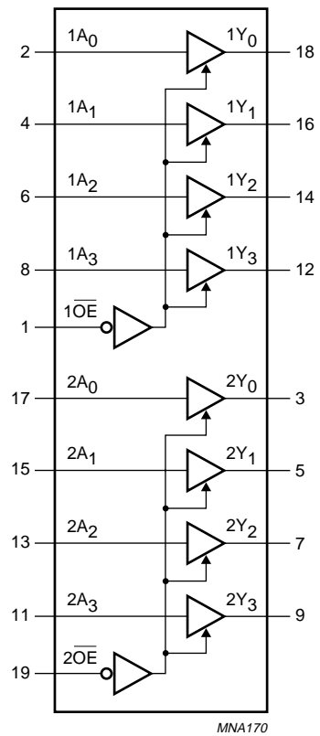
Fig.3 Logic diagram.
