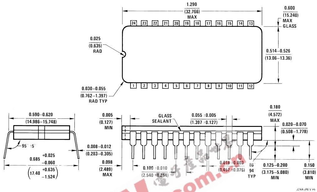
24-Lead Ceramic Dual-In-Line Package Number J24A
