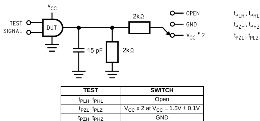
FIGURE 7. AC Test Circuit
