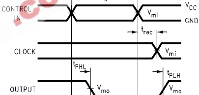
FIGURE 5. Propagation Delay, Pulse Width and t_{rec} Waveforms
