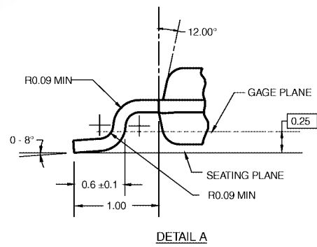
20-Lead Thin Shrink Small Outline Package, (TSSOP) JEDEC Package Number MTC20
