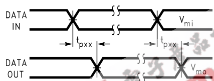
FIGURE 8. Waveform for Inverting and Non-Inverting Functions
