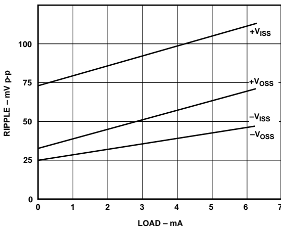
Figure 16a. Isolated Supply Ripple vs. Load (External 4.7\text{ }\mu\text{F} Bypass)
