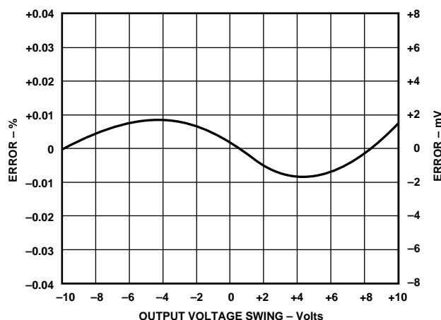
Figure 12. Gain Nonlinearity Error vs. Output
