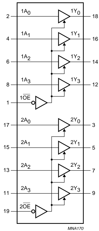
Fig.3 Logic diagram.
