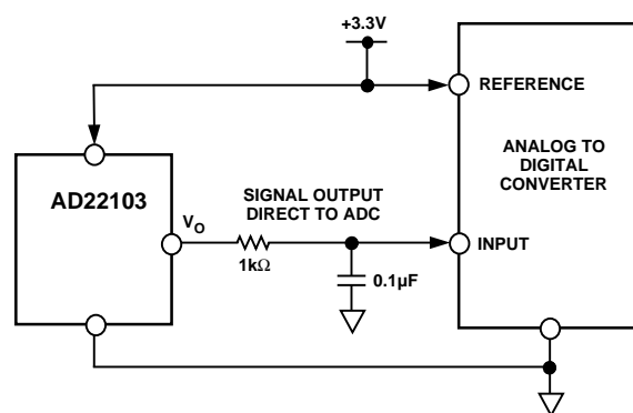
Figure 1. Application Circuit
