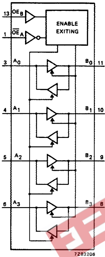
Fig.4 Functional diagram.
