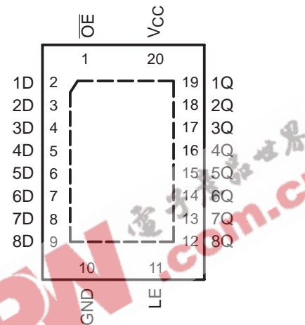
SN74LV573A . . . RGY PACKAGE (TOP VIEW)
