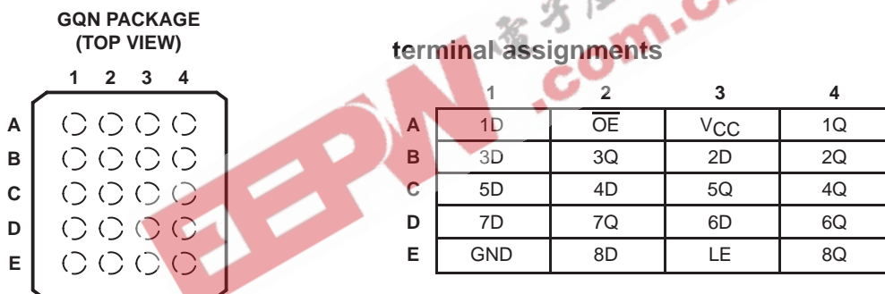
FUNCTION TABLE (each latch)
