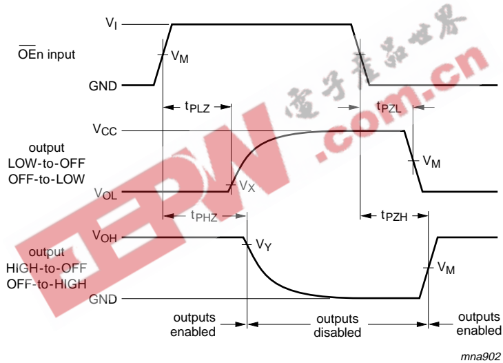
Fig 5. Propagation delay input (An) to output (Yn)
