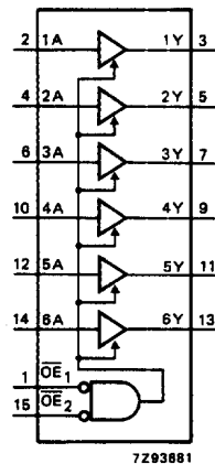
Fig.4 Functional diagram.
