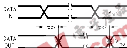
FIGURE 2. Waveform for Inverting and Non-Inverting Functions
