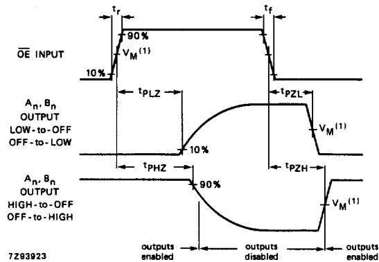
Fig.9 Waveforms showing the input \overline{\text{OE}} to output A n , B n 3-state enable and disable times.
