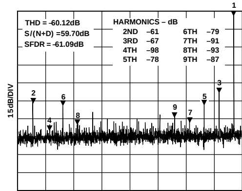
Figure 8. Typical FFT, f_{IN} = 1.450 MHz
