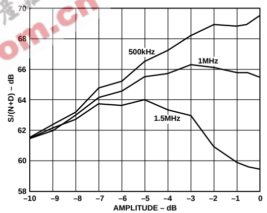
Figure 5. S/(N+D) vs. Amplitude
