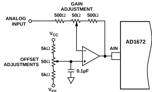
Figure 12. Offset and Gain Adjustment
