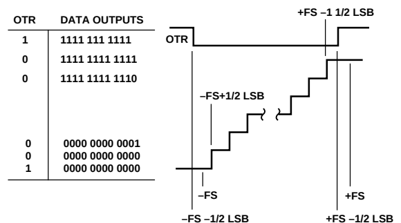
Figure 20. Output Data Format
