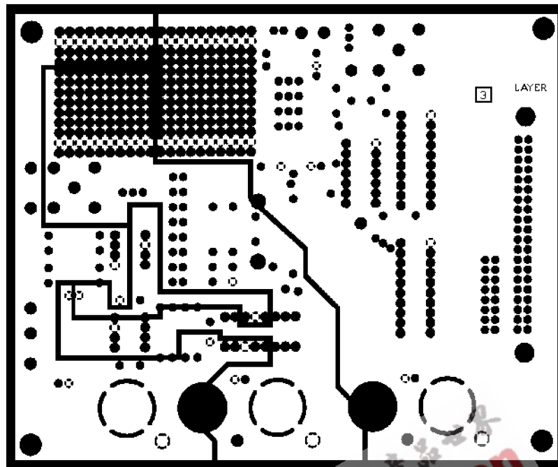
Figure 36. PCB Power Plane Layout for AD1672
