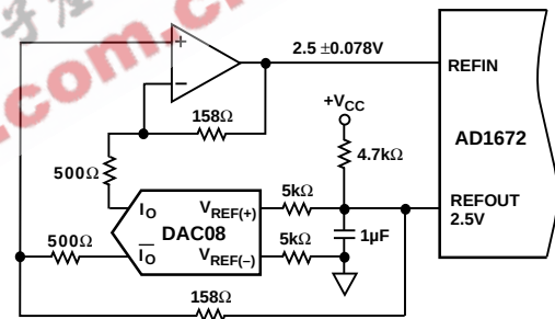
Figure 30. Gain Correction Using the DAC08
