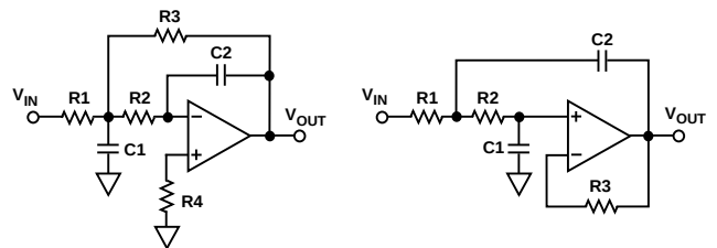
Figure 13. Sallen-Key and Multiple-Feedback Antialiasing Filter Topologies
