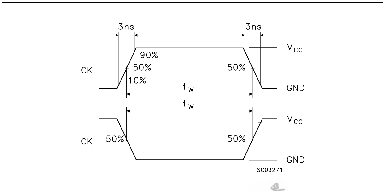
Figure 7: Waveform - Minimum Pulse Width ( f=1\text{MHz} ; 50% duty cycle)
