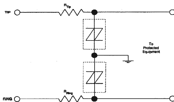
FIGURE 9 - UL 1459 & FCC Part 68 - Longitudinal Protection
