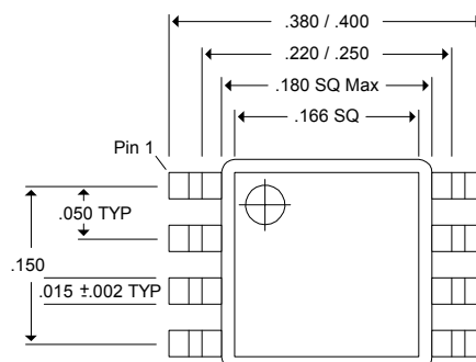
Figure 1. Package Drawings
