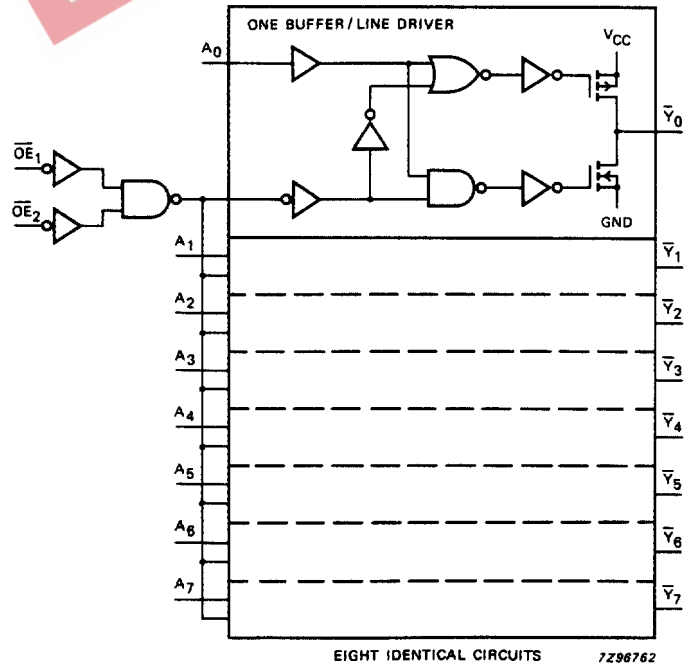
Fig.5 Logic diagram.
