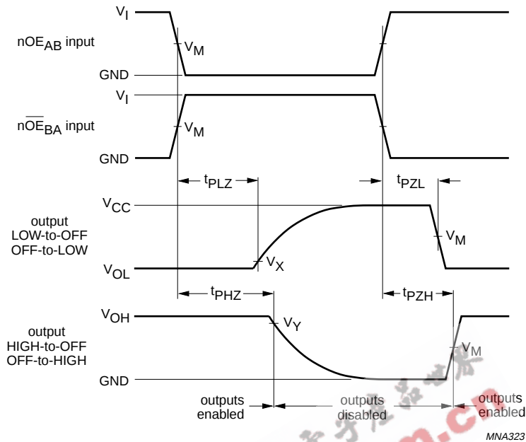
Fig.9 The OE inputs ( \overline{nOE_{AB}} , \overline{nOE_{BA}} ) to outputs nA_n , nB_n enable and disable times and the input rise and fall times.
