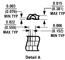
Ceramic Leadless Chip Carrier Package (E) Order Number 54LS11LMQB NS Package Number E20A
