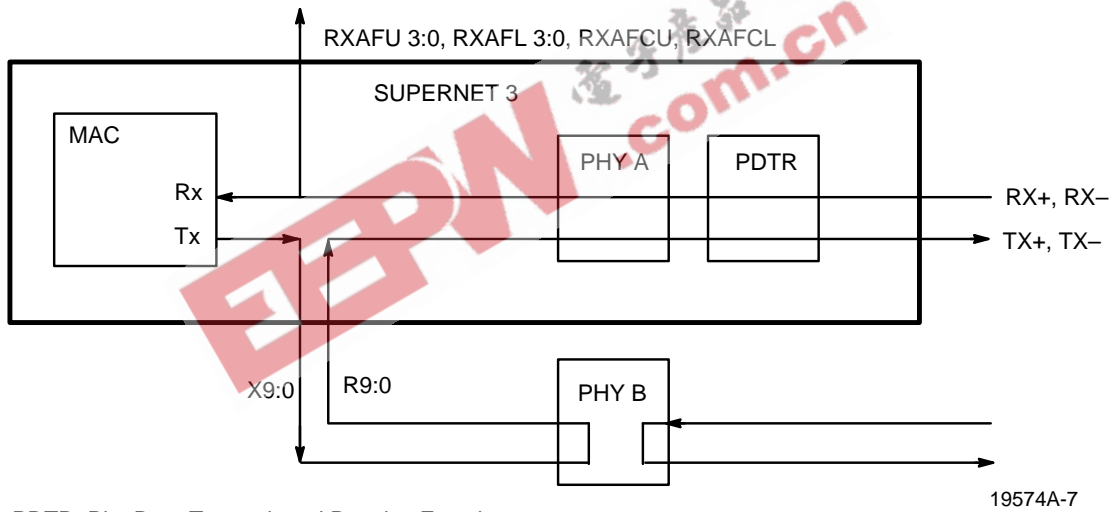
PDTR: Phy Data Transmit and Receive Functions
