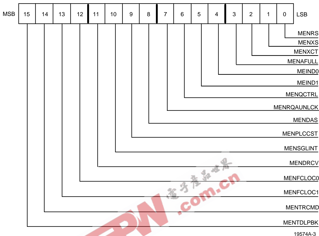
Figure 2. Register 3 (MDREG3) (NPADDR = 60h)
