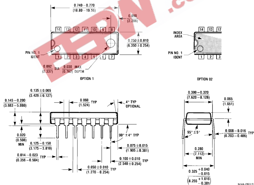
14-Lead Molded Dual-In-Line Package (N) Order Number DM74LS11N NS Package Number N14A
