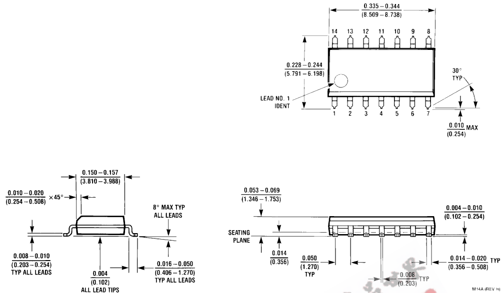
14-Lead Small Outline Molded Package (M) Order Number DM74LS11M NS Package Number M14A
