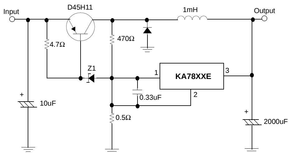
Figure 17. Switching Regulator
