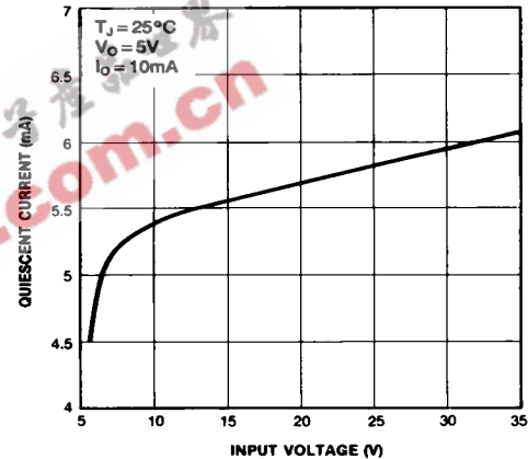
Figure 4. Quiescent Current
