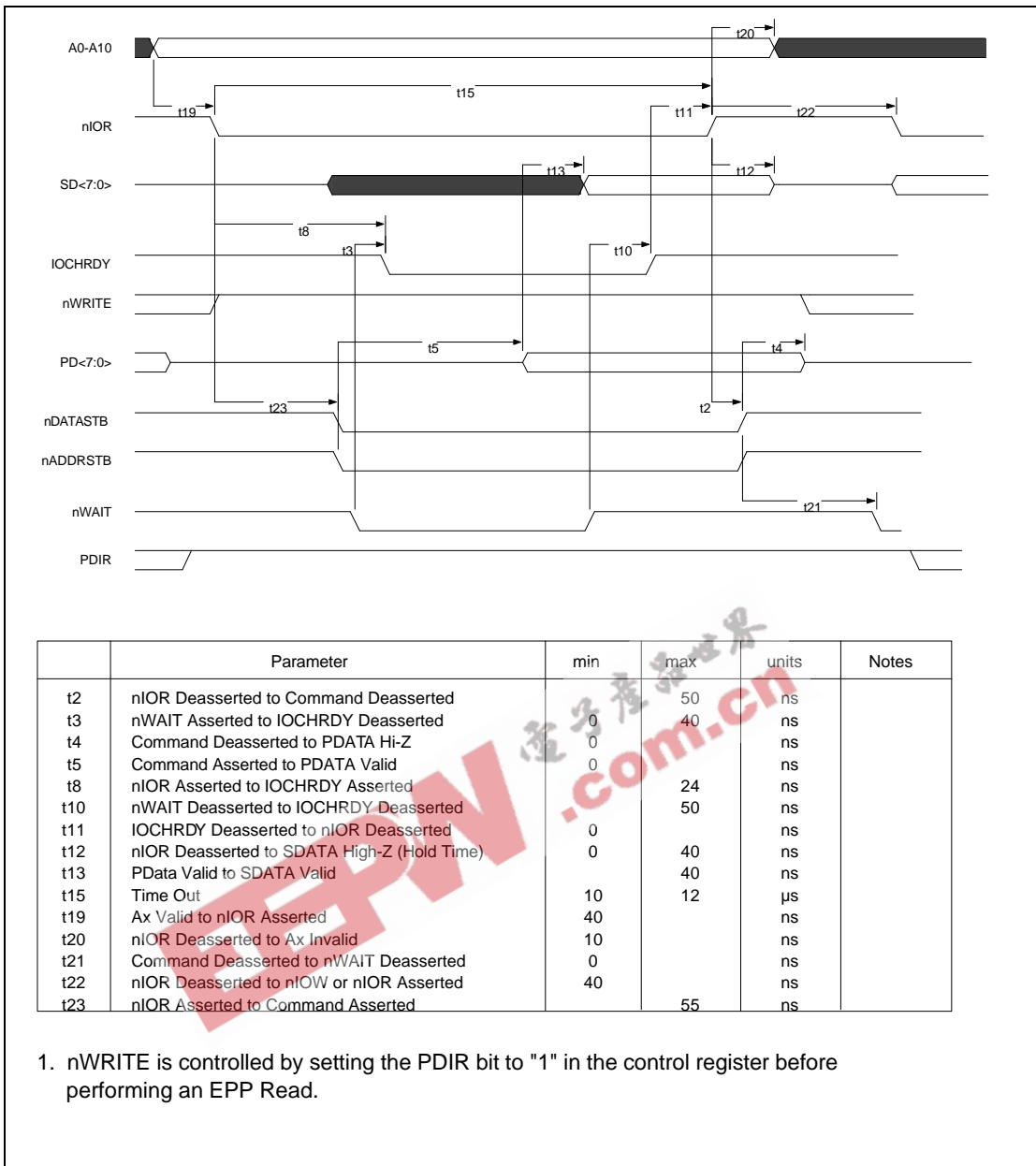
FIGURE 20 - EPP 1.7 DATA OR ADDRESS READ CYCLE
