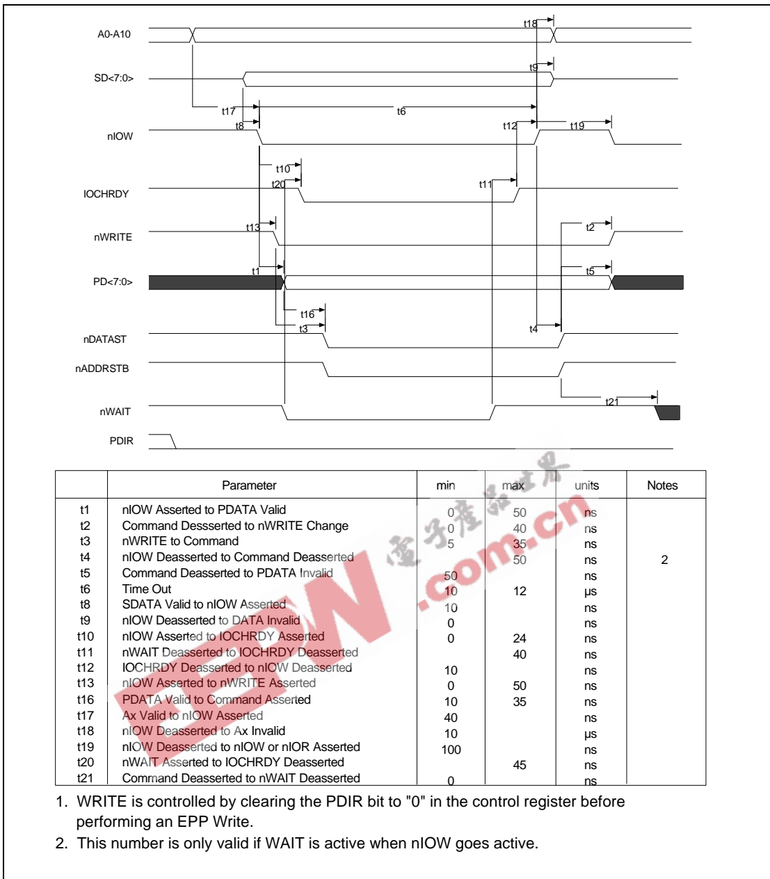
FIGURE 19 - EPP 1.7 DATA OR ADDRESS WRITE CYCLE
