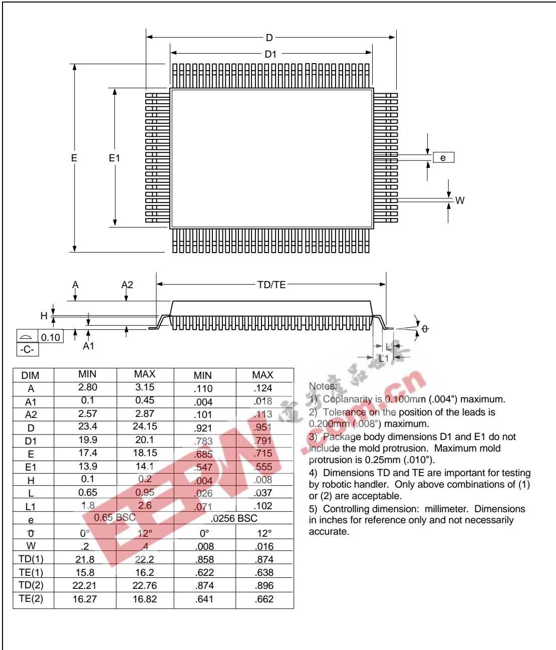
FIGURE 24 - 100 PIN QFP
