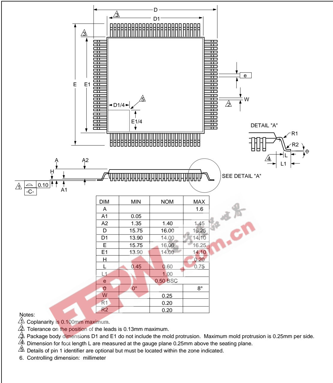
FIGURE 25 - 100 PIN TQFP
