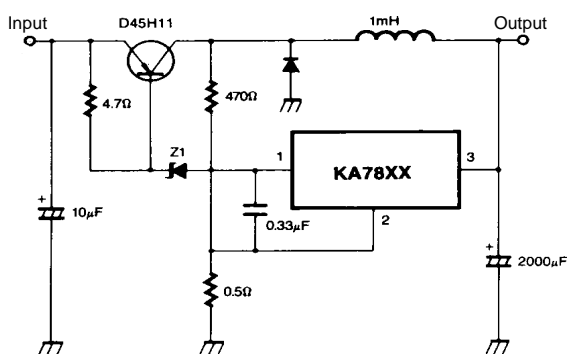
Figure 17. Switching Regulator
