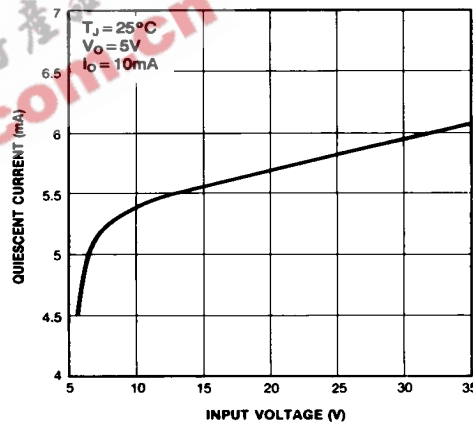
Figure 4. Quiescent Current
