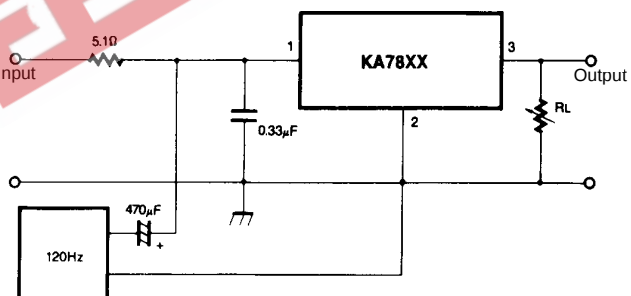
Figure 7. Ripple Rejection
