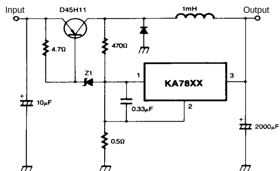
Figure 17. Switching Regulator
