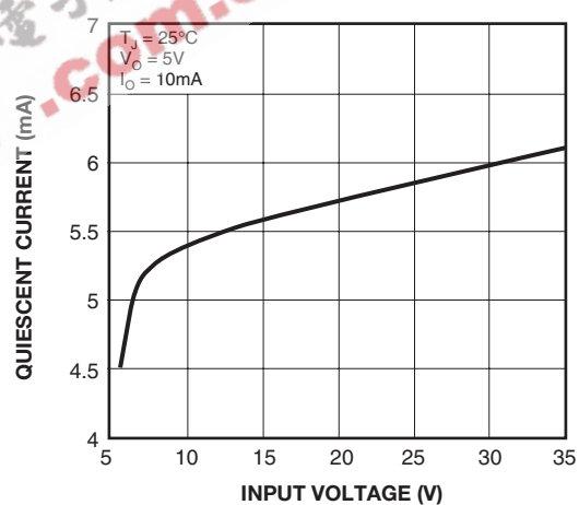
Figure 6. Quiescent Current
