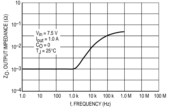
Figure 4. Output Impedance
