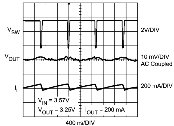
Output Voltage Ripple in Dropout ( V_{IN} = 3.75V , V_{OUT} = 3.25V , I_{OUT} = 200\text{mA} )
