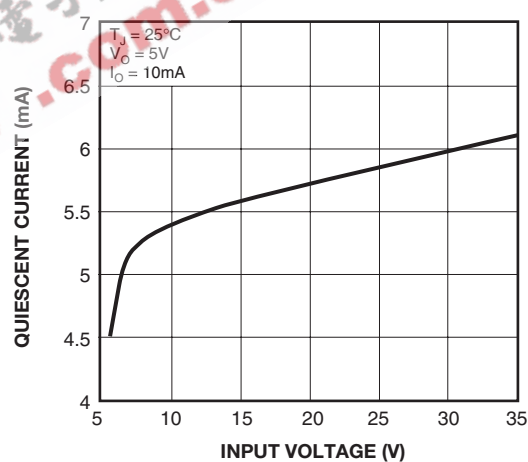
Figure 6. Quiescent Current
