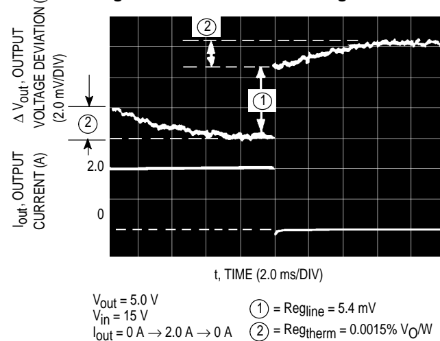
Figure 2. Load and Thermal Regulation
