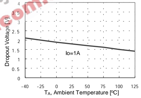
Figure 4. Dropout Voltage
