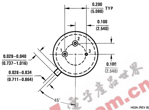
(TO-39) Metal Can Package NS Package Number H03A
