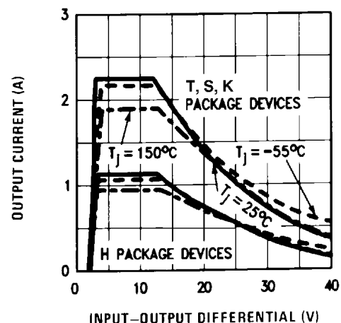
Current Limit
