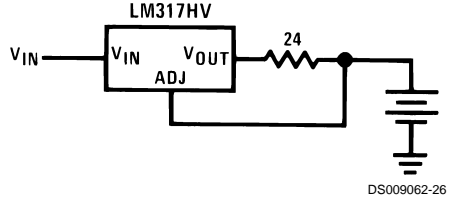
50 mA Constant Current Battery Charger
