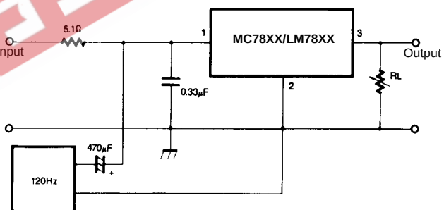
Figure 7. Ripple Rejection
