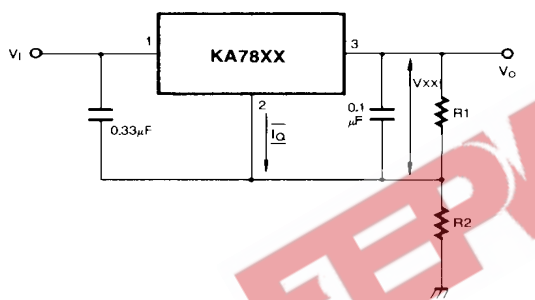
Fig. 10 Circuit for Increasing Output Voltage
