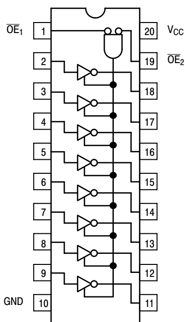
Figure 1. MC74AC540/74ACT540
