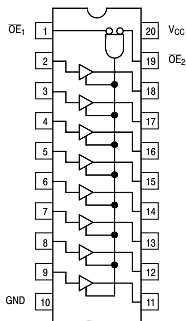
Figure 2. MC74AC541/74ACT541
